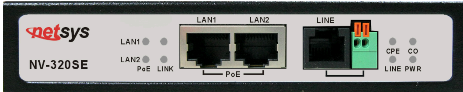
Figure 3.1 Front Panel
